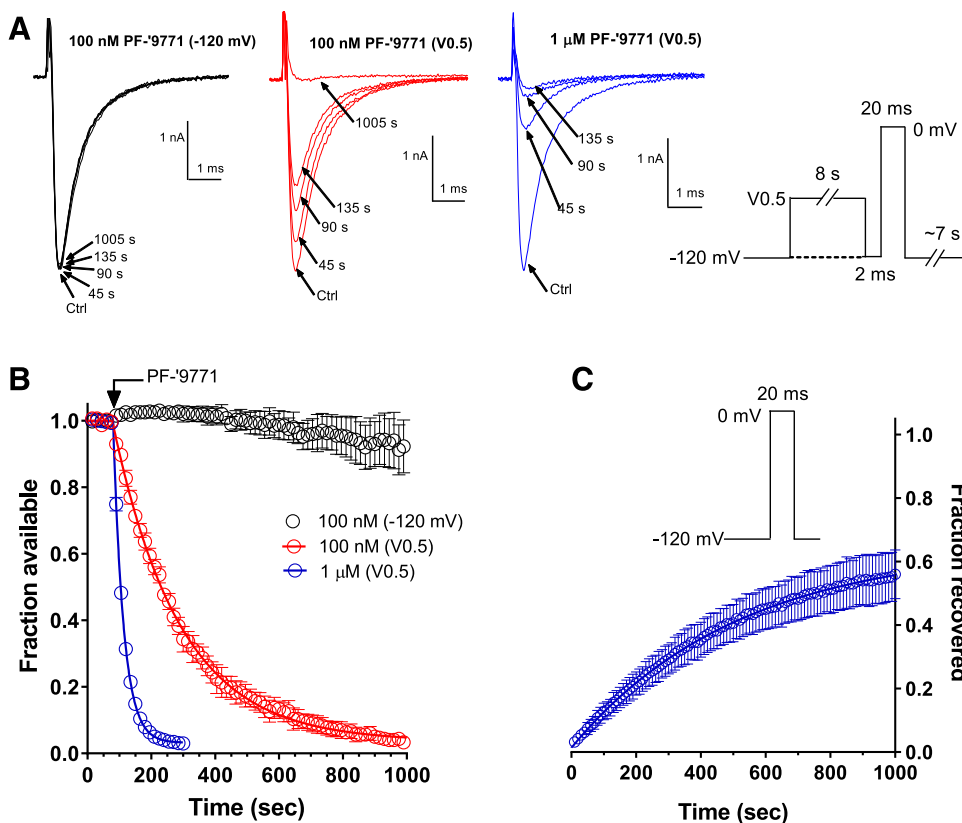
Fig. 1. Inhibition of human \text{Na}_v1.7 by PF-05089771 develops and recovers slowly. (A) Representative traces showing the time course of inhibition under the three different recording conditions. Inhibition by PF-05089771 was assayed against resting channels (steady holding at -120 mV) and a protocol in which channels were half-inactivated during 8-second prepulses delivered every 15 seconds from a steady holding voltage of -120 mV ( V_{0.5} of inactivation potential was determined empirically for each cell). The sweep interval for both protocols is 15 seconds. (B) Time course of inhibition for half-inactivated channels was dose dependent, reaching nearly complete block at both 100 nM ( n = 3 ) and 1 \mu\text{M} ( n = 9 ); however, block was minimal for resting channels ( n = 4 ). (C) Recovery from block after washout of 1 \mu\text{M} PF-05089771 using the tonic protocol (inset) is slow and incomplete ( n = 5 ).
