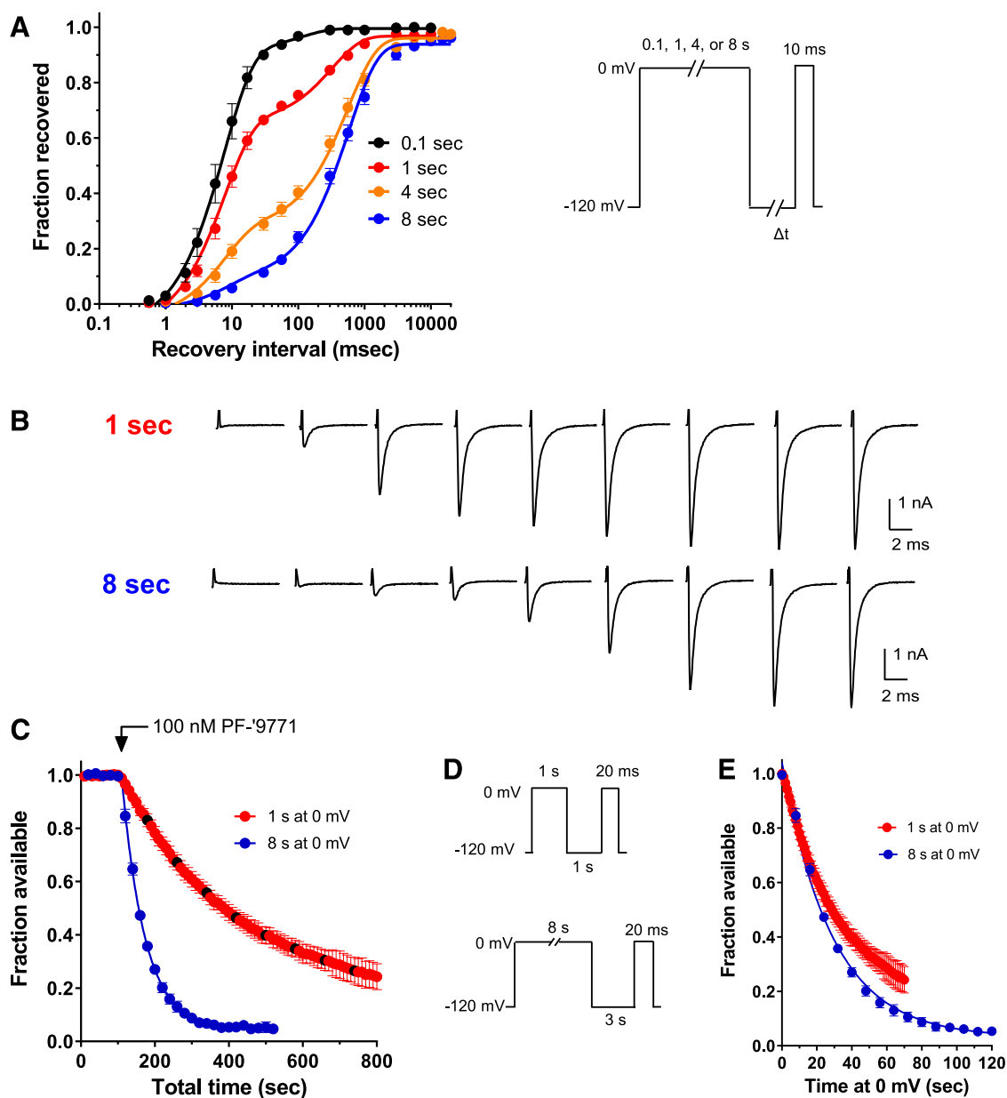
Fig. 3. Time course of block by PF-05089771 is independent of the availability of kinetically defined inactivated states. (A) Recovery from inactivation was assessed after a conditioning depolarizing pulse to 0 mV for 0.1, 1, 4, and 8 seconds in the absence of PF-05089771 ( n = 4, 4, 4, and 5, respectively). A variable recovery interval at -120 mV followed each step to 0 mV. After the recovery interval, a 10-ms test pulse at 0 mV assessed the fraction of available current. As the conditioning pulse is increased from 0.1 to 8 seconds, a larger fraction of channels enter a slowly recovering state. (B) Individual traces from a single representative cell showing recovery from inactivation after either a 1-second (top traces) or an 8-second (bottom traces) pulse to 0 mV. The pulses represent the recovery intervals from 1 ms to 10 seconds in half-log intervals. (C) Onset of block by 100 nM of PF-05089771 was measured using a short (1 second, n = 5 ) or long (8 seconds, n = 7 ) inactivating conditioning pulse to 0 mV using the protocols shown in (D). The black dots overlaying the red data points represent the time-matched equivalent at 0 mV compared with blue data points (i.e., every 8 seconds). (D) A fixed recovery interval of 1 and 3 seconds at -120 mV (which allows for >90\% of the current to recover) was used for the 1- and 8-second conditioning pulse, respectively. Sweep intervals of 10 and 20 seconds were used with the 1- and 8-second conditioning pulses, respectively. (E) Replotting as the amount of block as a function of the total time spent at 0 mV uncovers a similar time course of inhibition between the two protocols ( \tau = 31 \pm 1 versus 32 \pm 4 seconds for the 8- and 1-second conditioning steps, respectively; P > 0.05 by unpaired t test).
