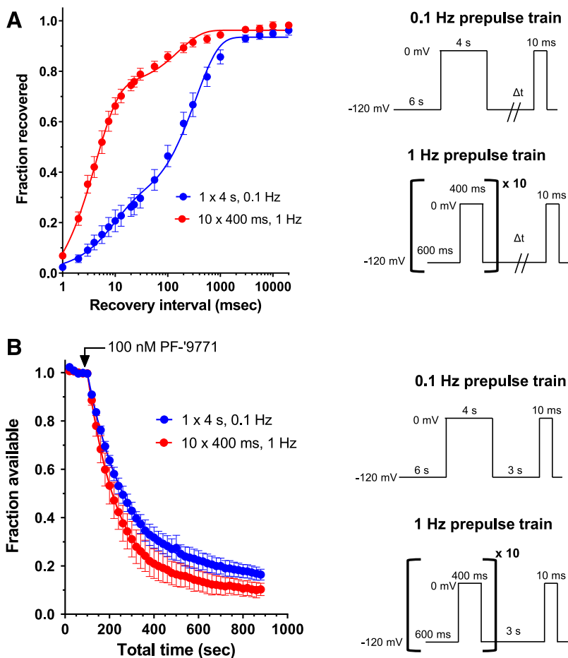
Fig. 4. Onset of inhibition develops over similar time course using different conditioning trains with equal time at 0 mV. (A) Recovery from inactivation was assessed after a conditioning prepulse train to 0 mV at a frequency of 1 Hz ( n = 5 ) and 0.1 Hz ( n = 4 ) in the absence of PF-05089771. (B) Onset of block by 100 nM of PF-05089771 ( n = 3 , each) was measured using both protocols but with a fixed recovery interval of 3 seconds at -120 mV and a sweep interval of 20 seconds. The onset of block is similar with both protocols ( \tau = 141 \pm 23 seconds for the 10 \times 400 ms, 1 Hz and 178 \pm 16 seconds for the 1 \times 4 seconds, 0.1 Hz, n = 3 each; P > 0.05 by unpaired t test), despite the \sim 3.4 -fold difference in relative availability of slow inactivated channels with the 0.1-Hz conditioning stimulus.
