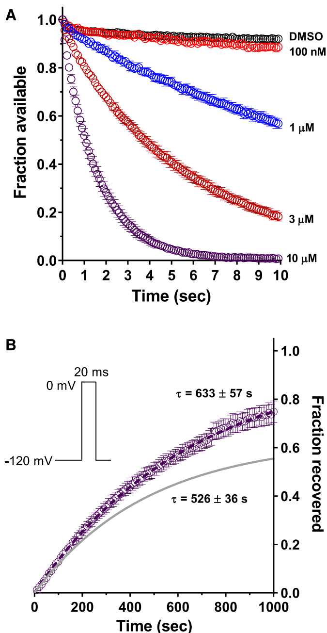
Fig. 2. By using brief depolarizations, PF-05089771 exhibits use dependence only at very high concentrations. (A) Use-dependent inhibition was examined by employing a standard high-frequency pulse train consisting of 100 steps (20 ms) to 0 mV at a rate of 10 Hz. The 10-Hz train was tested against the vehicle control (0.1% DMSO, n = 24 ) and PF-05089771 at 100 nM ( n = 5 ), 1 \mu M ( n = 5 ), 3 \mu M ( n = 5 ), and 10 \mu M ( n = 9 ). (B) After complete block with the 10-Hz train in the presence of 10 \mu M PF-05089771, recovery was assessed using a tonic protocol (inset) while washing out the compound ( n = 8 ). The gray line is the curve fit from Fig. 1C, showcasing the similar rate but different extent of recovery from block.
