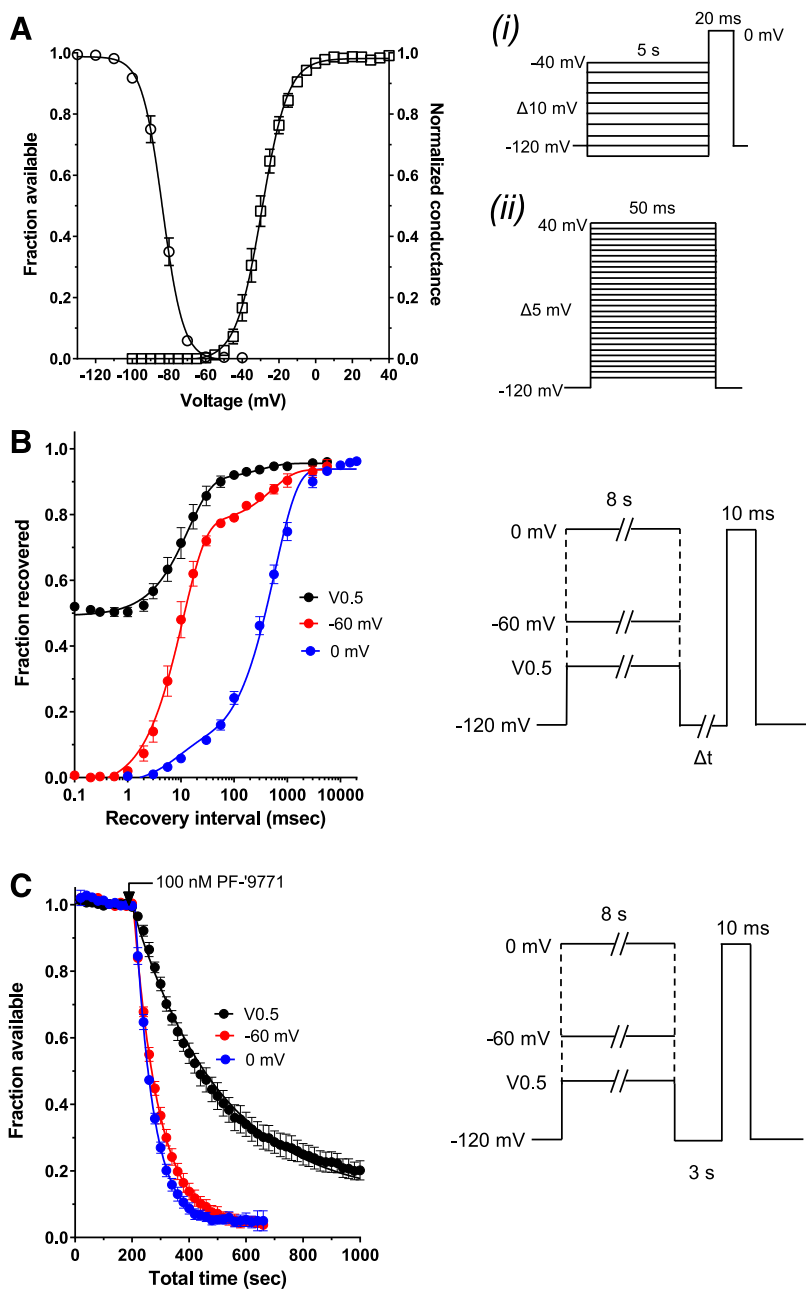
Fig. 5. Onset of inhibition develops over similar time course from closed- and open-state inactivation. (A) Activation and steady-state inactivation curve show minimal overlap. The voltage dependence of steady-state inactivation (circles) was determined using the protocol shown in (i) with a V0.5 of -83.5 \pm 0.5 mV ( n = 9 ). The voltage-dependence of activation (squares) was determined using the protocol shown in (ii) with a V0.5 of -29.3 \pm 0.3 mV ( n = 11 ). (B) Recovery from inactivation was assessed after a conditioning pulse at 0 mV (channels inactivated through open state, n = 5 ), -60 mV (channels predominantly inactivated through closed state, n = 3 ) or the V0.5 of inactivation (as determined empirically for each cell, n = 3 ). For the conditioning pulses to -60 and 0 mV, 100% of the channels are inactivated. The rate of recovery for the -60 mV and V0.5 conditioning steps have a considerably larger fast component compared with the conditioning step to 0 mV. Likewise, the recovery from the V0.5 conditioning pulse is predominantly fast. (C) Onset of block by 100 nM of PF-05089771 was measured using each protocol with a fixed 3-second recovery interval at -120 mV and a 20-second sweep interval. The rate of block is similar for the 0 mV ( n = 7 ) and -60 mV ( n = 5 ) protocols ( P > 0.05 by ANOVA), despite having dramatically different recovery profiles; however, the onset of block is dramatically slower using the V0.5 potential ( P < 0.01 by ANOVA and Tukey's multiple comparison test, n = 6 ).
